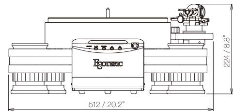
Overall Dimensions (unit: mm/inch)
