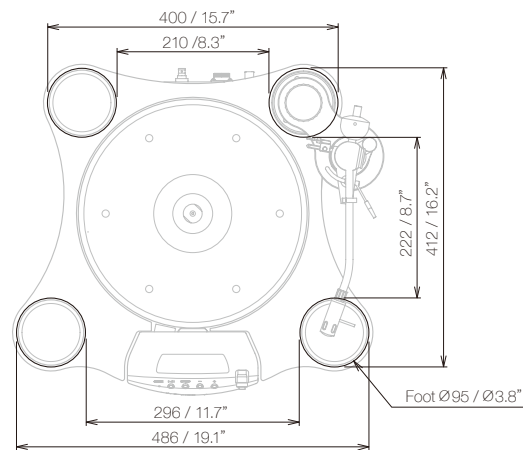
Foot positions (unit: mm/inch)
