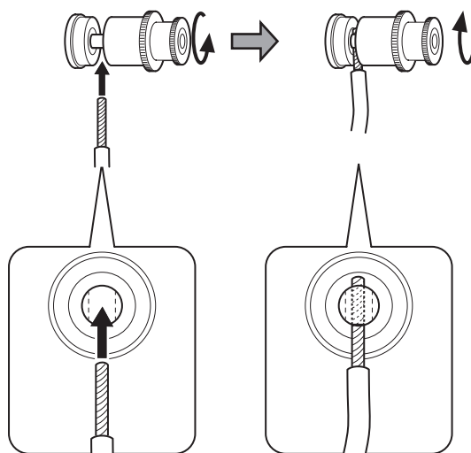
Cross-sections
